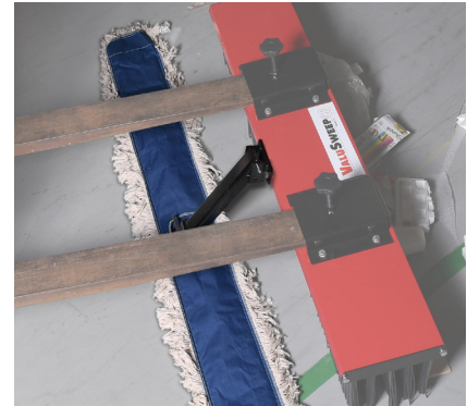
VSB-048 Broom equipped with optional DMP-060-1 Dust Mop Kit.
