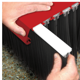
VBK-048/VBK-060 REPLACEMENT BRUSH KIT
